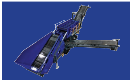
2 Way Split Configuration - An easy retrofit kit requiring minimal downtime for installation.
